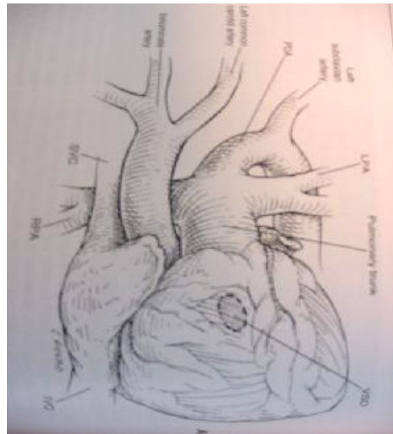
Fig. 1. Schematic view of interrupted aortic arch type 2
